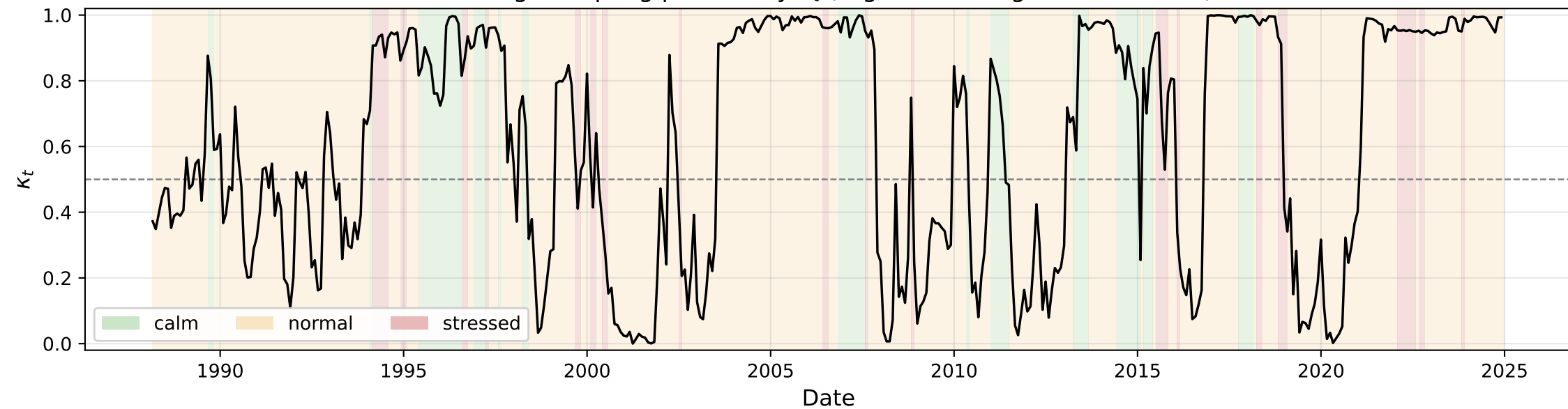
Average coupling probability \kappa_t (regime shading, 0.5 reference)
